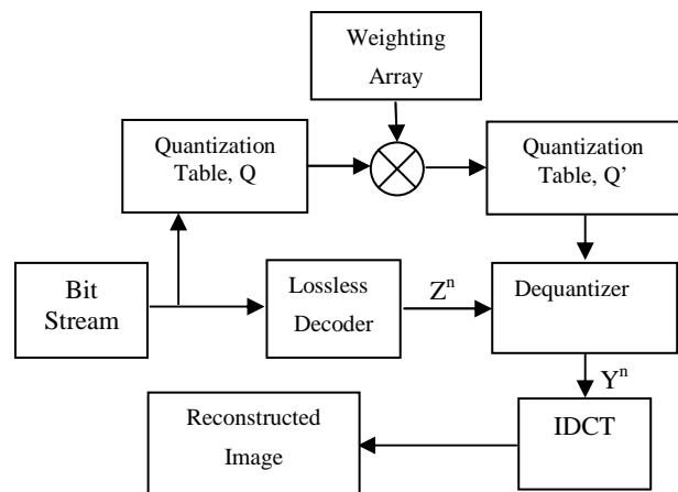
Figure 1. JPEG Decoder with image enhancement function Note \otimes is a point-by-point multiplication.
