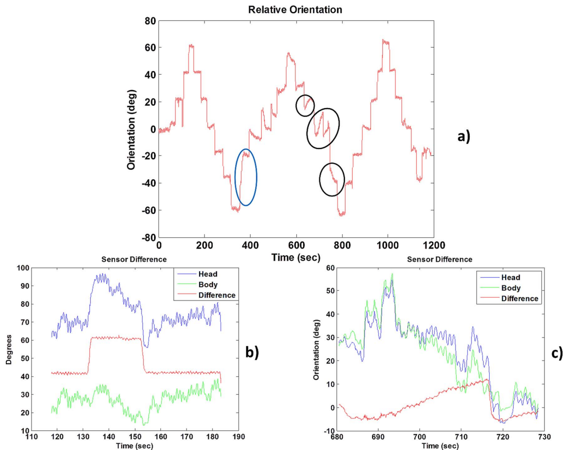
Figure 3. Relative orientation in degrees between the two inertial measurement units (IMUs) in Experiment 1a. (a) Steps of 20^\circ are clearly shown in the relative orientation output. Note that after 300 s the system starts drifting (experiencing uncorrelated noise), and there is an error of about 20^\circ . The step in the blue ellipse should be 20^\circ increment and not 40^\circ , and the sections of the output highlighted by the black ellipses should appear flat in the plot (constant); only a few of them are marked for the sake of clarity. (b) Orientation output of the head and body sensors for a 60-s segment of the recording around the peak at 140 s on plot (a). The net head rotation is obtained by subtracting the output of the body motion sensor from the head motion sensor. Although both appear to be very noisy, the noise is highly correlated, and the differential signal provides relative orientation, which is close to the ground truth. (c) Orientation output of the head and body sensors for a 50-s segment of the recording, starting at 680 s on plot (b), showing details of uncorrelated noise in the two sensors. In this case, the differential output does not help, and the measured net head rotation increases when it should have been flat.
